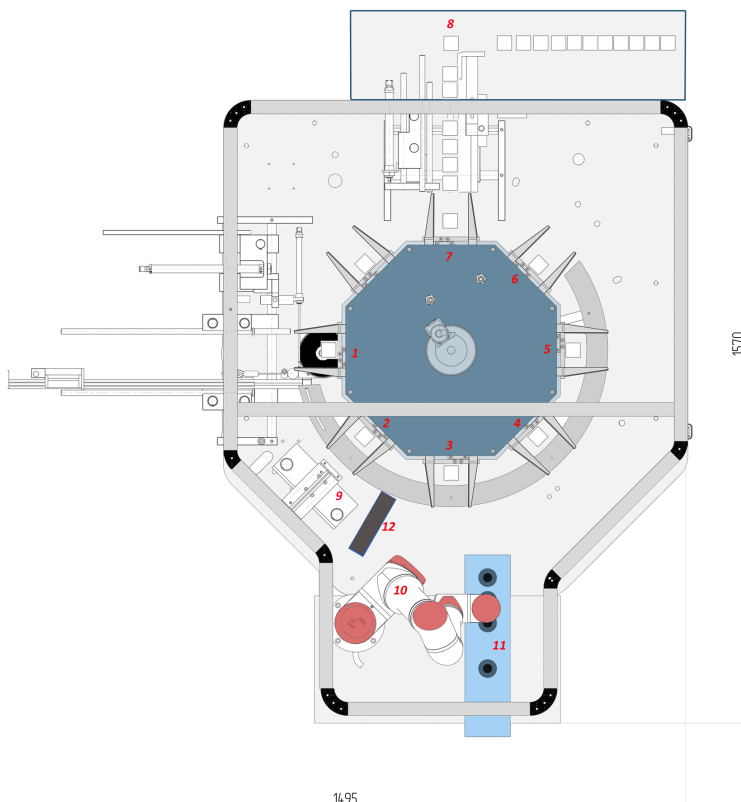
Layout C4/S with Robot Arm
